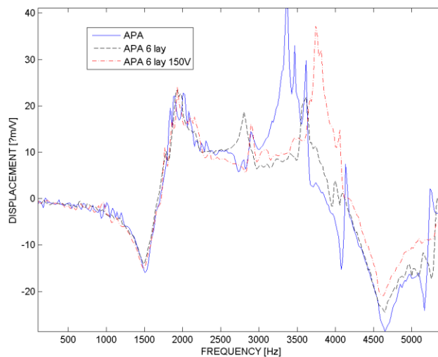
Fig. 10. Actuator vibration transfer
