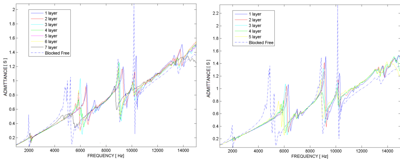
Fig. 9. Admittance curves for 130 \mu\text{m} (to the left) and 300 \mu\text{m} (to the right) thick VEM
