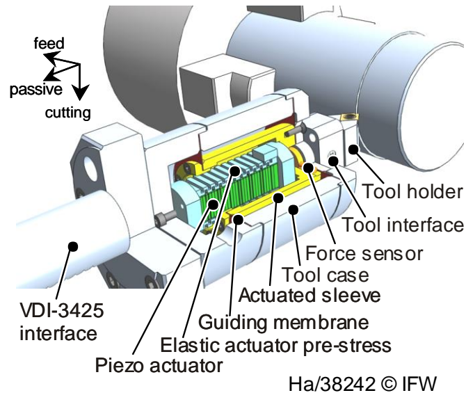
Fig. 2. Active tool adaptor based on PPA®
