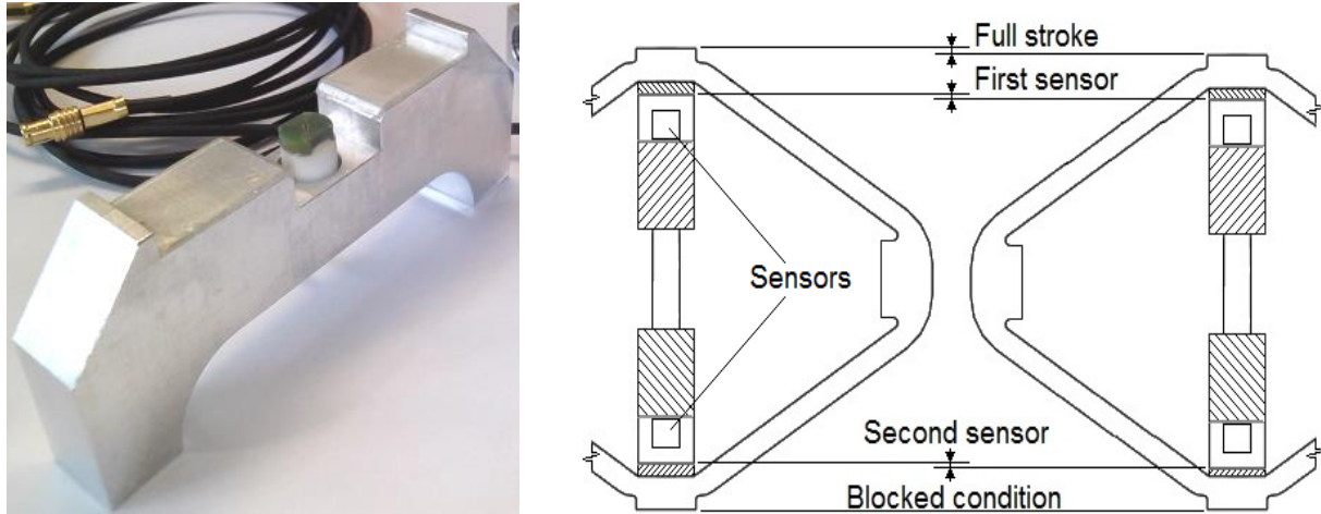
Fig. 12. View of the sensor in the one part of support and the principle of the displacement measurement by the eddy current sensors
