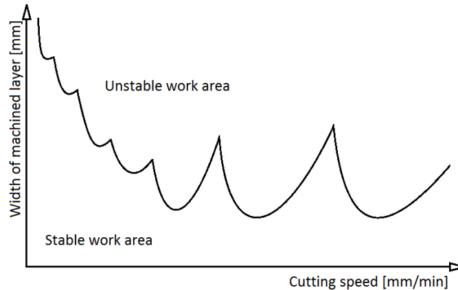
Fig. 1. Stability lobe diagram of typical machine tool
