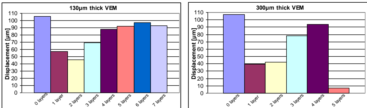
Fig. 8. Stroke measurement for 130\mu m (to the left) and 300\mu m (to the right) thick VEM
